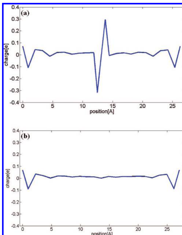
Figure 3. Partial charge distribution for atoms on SW-defective (5,5) boron nitride nanotube (BNNT) (a) and on a nondefective (5,5) BNNT (b) along the tube axial direction. The BNNT starts at 0 Å in the axial direction.
