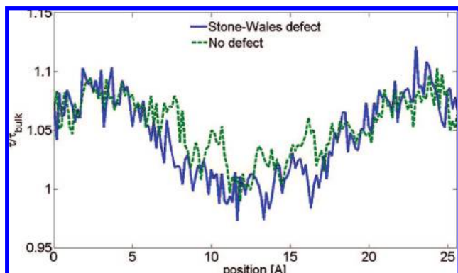
Figure 4. Residence time of water along the tube axial direction in the nondefective (dashed line) and SW-defective (solid line) (5,5) BNNT. The BNNT starts at 0 Å in the axial direction.
