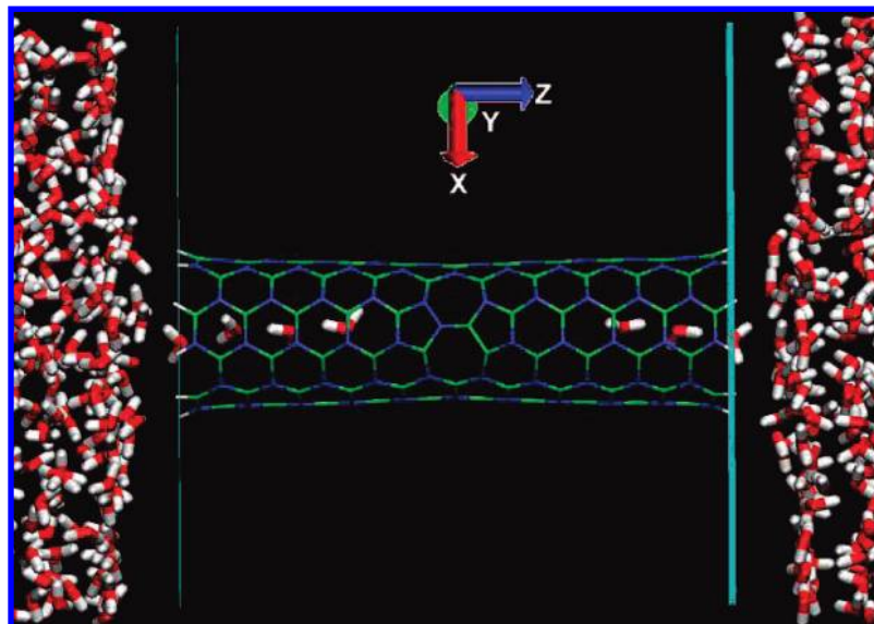
Figure 1. Visualization of a broken single-file water chain in a (5,5) BNNT with Stone–Wales (SW) defects in the center of the tube.
