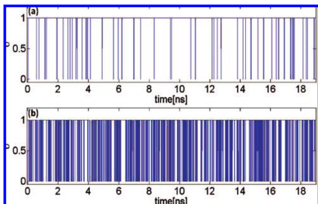
Figure 2. Phase transition v(t) of water inside the (a) nondefective and (b) SW-defective (5,5) boron nitride nanotube (BNNT).
